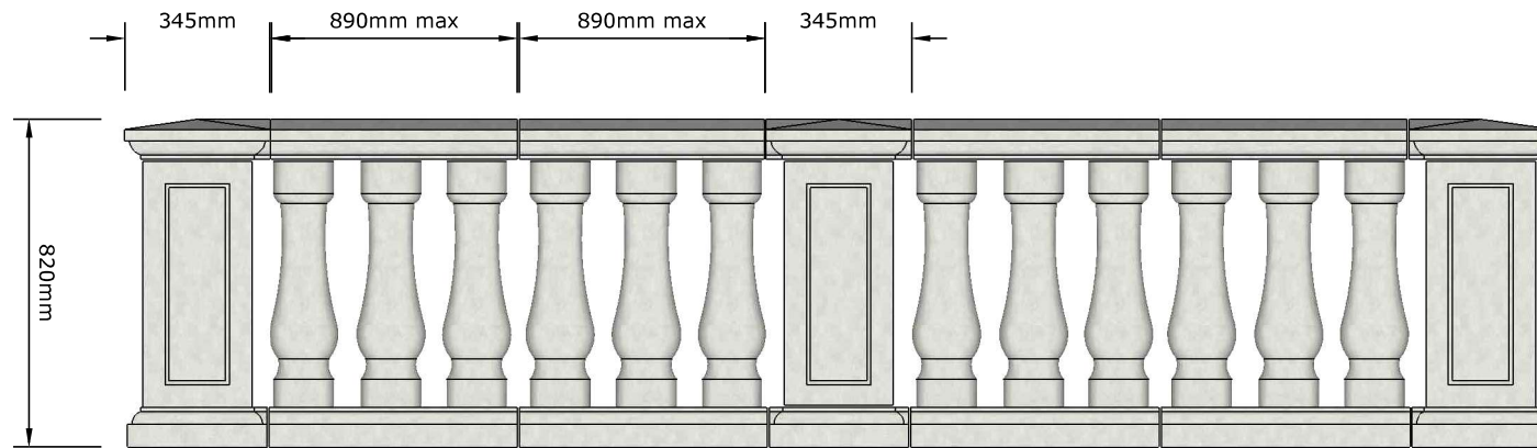
Front Elevation
