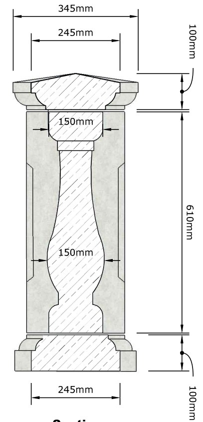
Section
