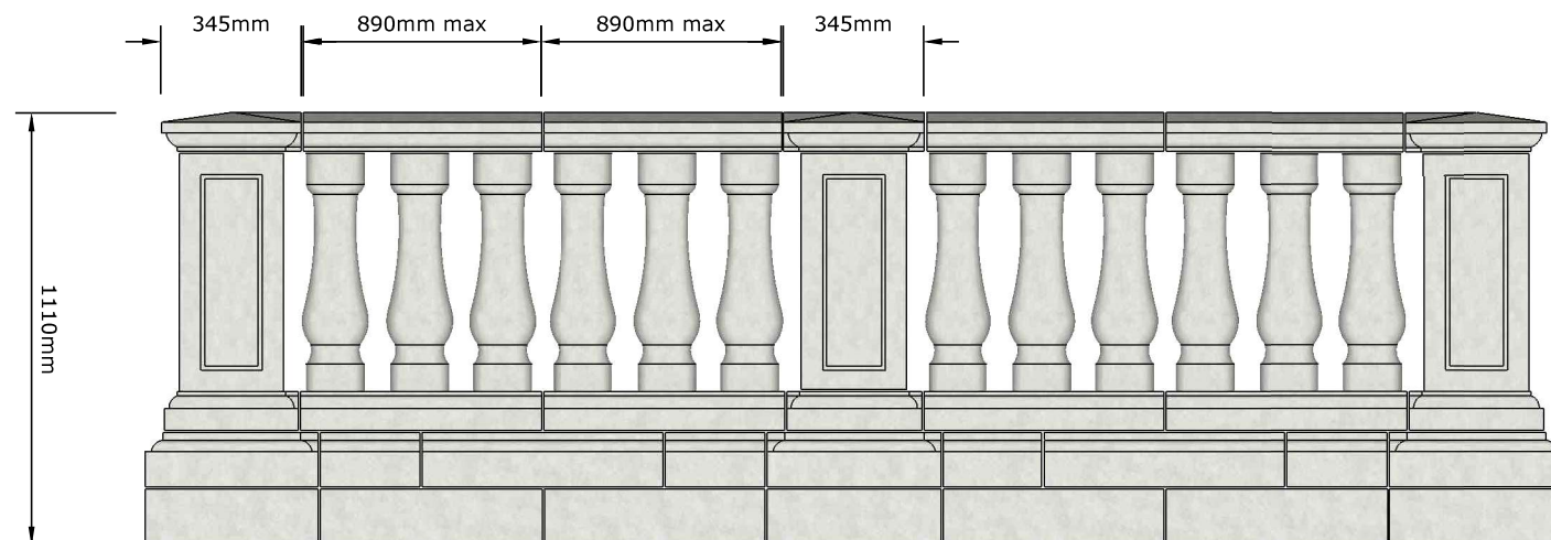
Front Elevation
