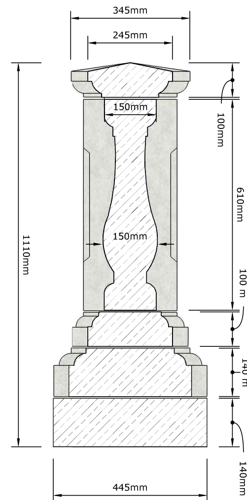
Section
