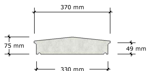
COPING TYPE 4 (310)
