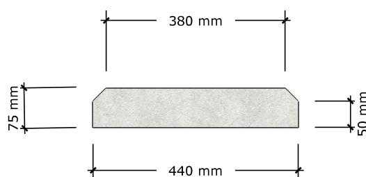
COPING TYPE 8 (430)
