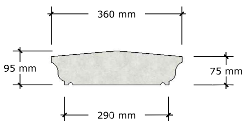
COPING TYPE 5 (275)
