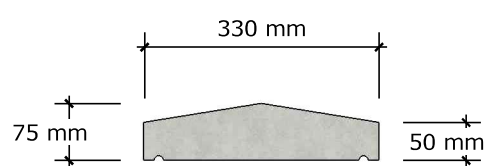
COPING TYPE 3 (310)
