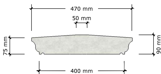
COPING TYPE 7 (390)
