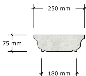
COPING TYPE 6 (160)
