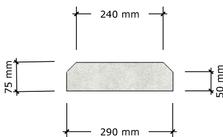
COPING TYPE 8 (290)
