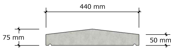
COPING TYPE 3 (430)
