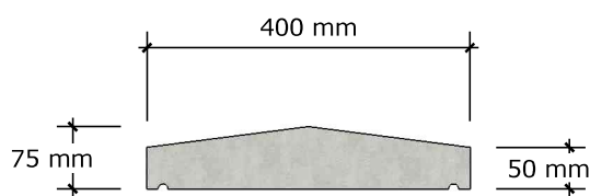
COPING TYPE 3 (390)
