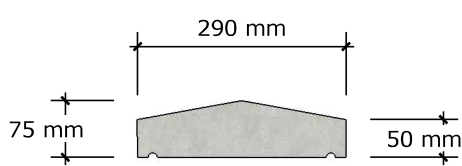
COPING TYPE 3 (275)
