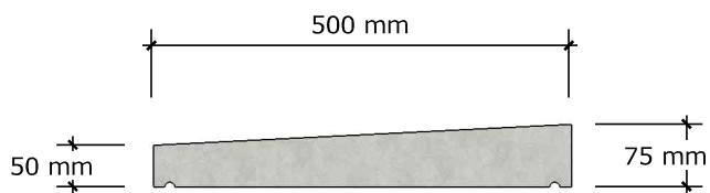
COPING TYPE 2 (500)
