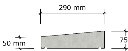
COPING TYPE 2 (275)
