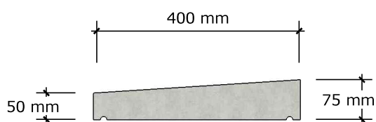
COPING TYPE 2 (390)
