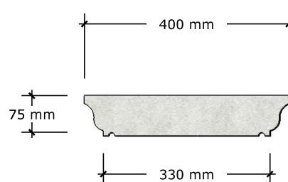
COPING TYPE 6 (310)
