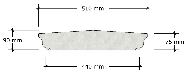
COPING TYPE 5 (430)
