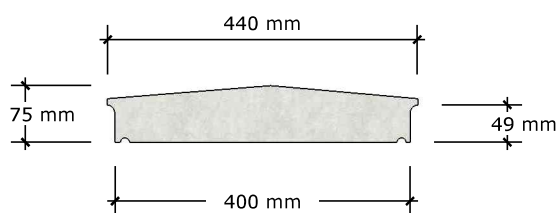
COPING TYPE 4 (390)
