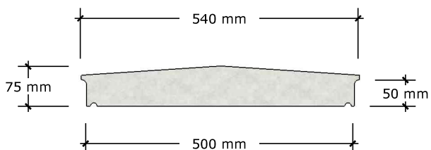
COPING TYPE 4 (500)
