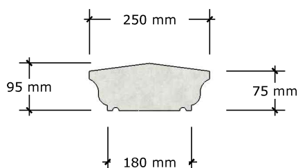
COPING TYPE 5 (160)
