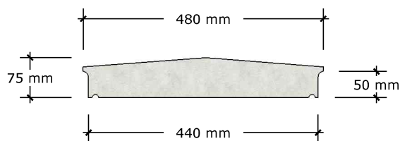
COPING TYPE 4 (430)
