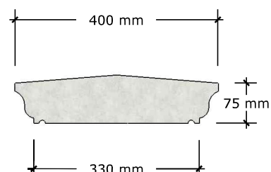
COPING TYPE 5 (310)
