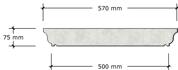
COPING TYPE 6 (500)
