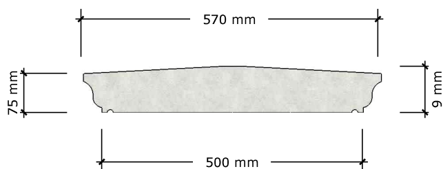
COPING TYPE 7 (500)
