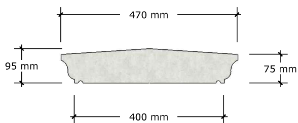
COPING TYPE 5 (390)
