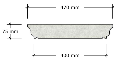
COPING TYPE 6 (390)
