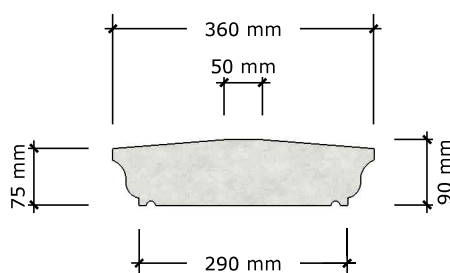
COPING TYPE 7 (275)
