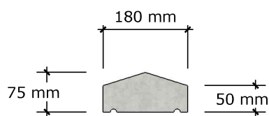
COPING TYPE 3 (160)
