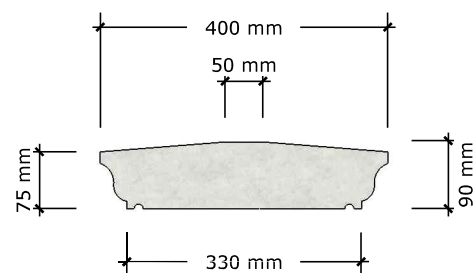
COPING TYPE 7 (310)
