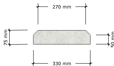
COPING TYPE 8 (310)
