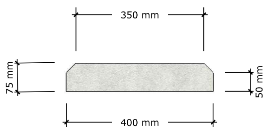
COPING TYPE 8 (400)
