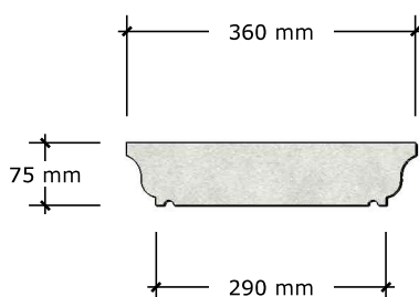
COPING TYPE 6 (275)
