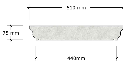
COPING TYPE 6 (430)
