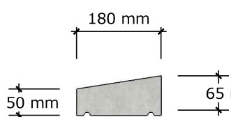
COPING TYPE 2 (160)
