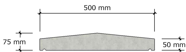
COPING TYPE 3 (500)
