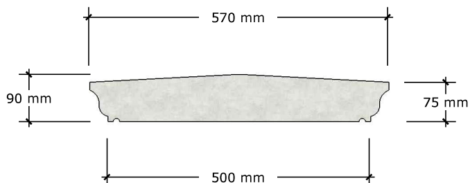
COPING TYPE 5 (500)
