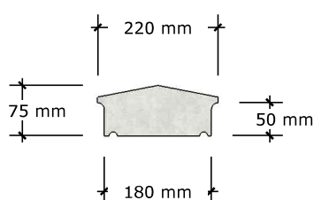
COPING TYPE 4 (160)
