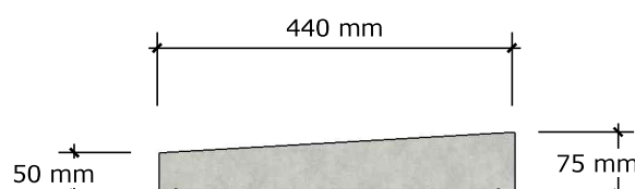
COPING TYPE 2 (430)
