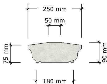
COPING TYPE 7 (160)
