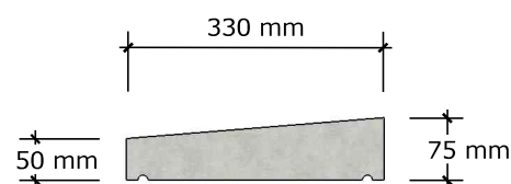
COPING TYPE 2 (310)
