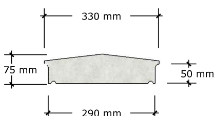
COPING TYPE 4 (275)
