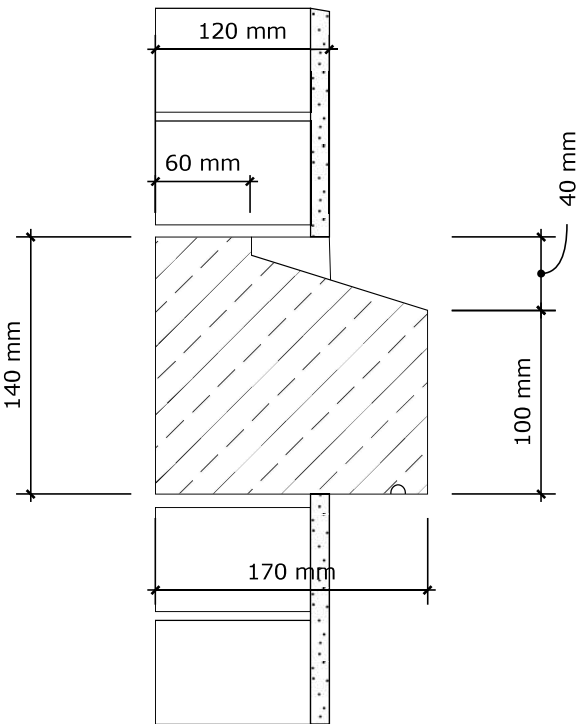
Cill Section in Render
