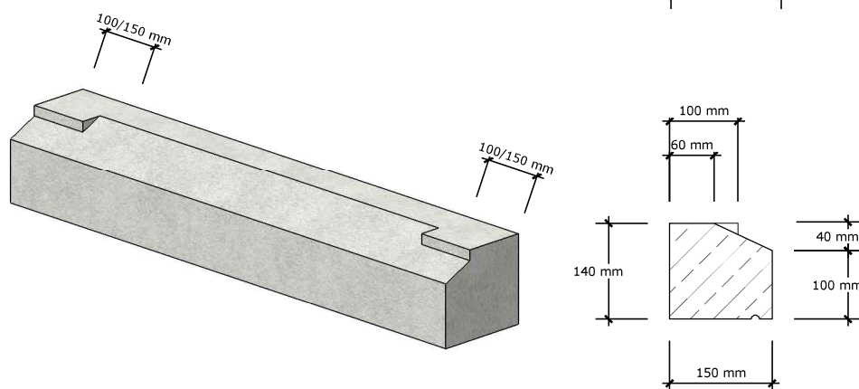
CILL TYPE.2 MAX LENGTH 1500mm 38kg /m
