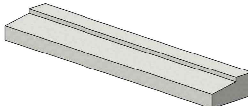
CILL TYPE.2-Slip MAX LENGTH 1500mm 38kg/m
