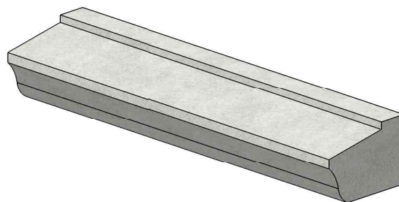
CILL TYPE.Regency-Slip MAX LENGTH 1500mm 46kg/m
