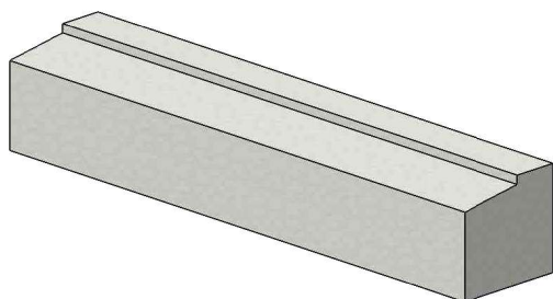
CILL TYPE.2-Slip MAX LENGTH 1500mm 38kg/m
