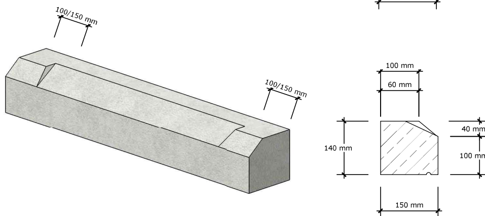
CILL TYPE.3 MAX LENGTH 1500mm 38kg /m
